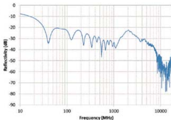
DSH-1250H DuraSorb™ Polystyrene Hybrid Absorber Typical Reflectivity
